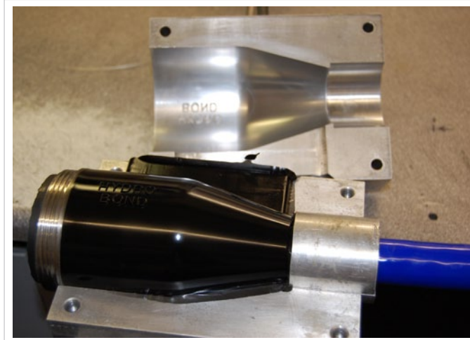
Breakout mould / harness manufacturing
